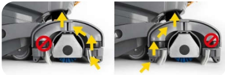
Alternate twin squeegee system (patented)
